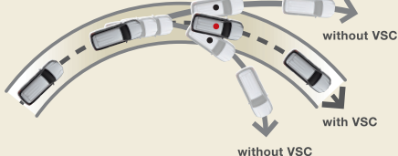
Vehicle Stability Control (VSC)
