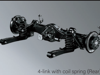
4-link with coil spring (Rear)
