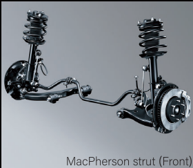
MacPherson strut (Front)
